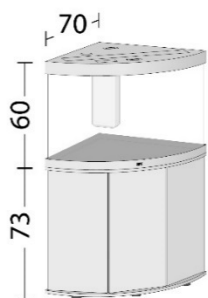
Maße: 98,5x70x60/73cm | ca. 190L 2x 14W LED (590mm) | Bioflow M Eccoflow 600 | AquaHeat Pro 200W
