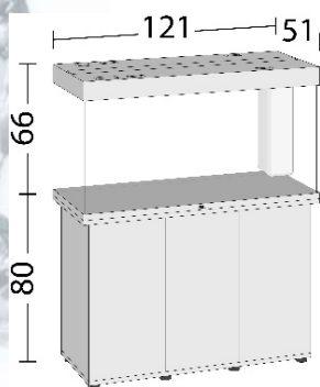
Maße: 121x51x66/80cm | ca. 350L 2x 29W LED (1047mm) | Bioflow L Eccoflow 1000 | AquaHeat Pro 300W
